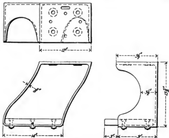
Figs. 3759-3761. Lower Step.
